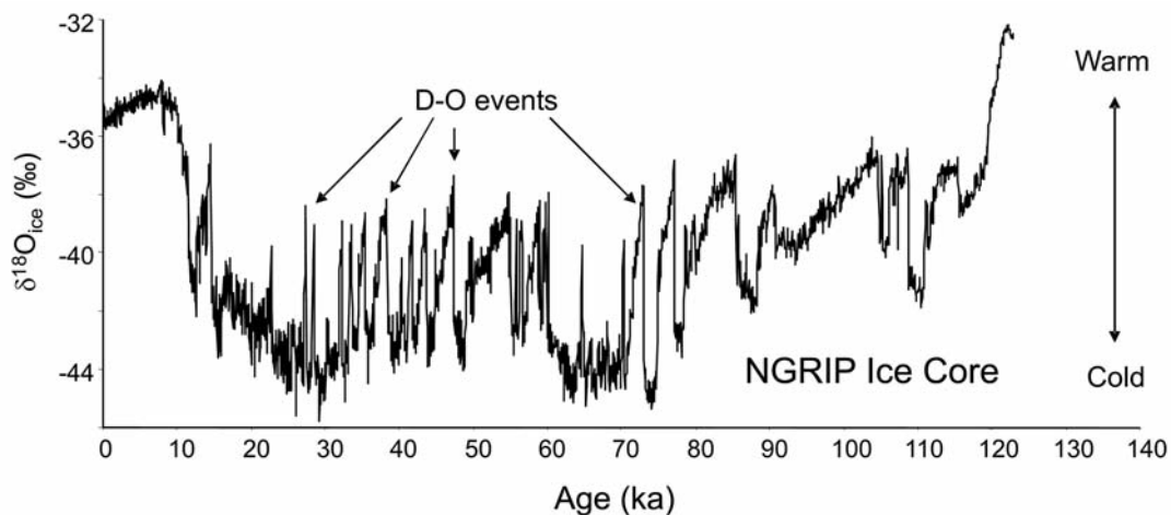
Fig. 1: Oxygen isotope record from the Greenland NGRIP ice core [NGRIP Project Members 2004], a proxy for air temperature changes. The high-resolution NGRIP record spans the last 123,000 years and reveals pervasive century- to millennial-scale variability. Rapid warming during the Dansgaard-Oeschger (D-O) events of the last glacial appears to have occurred over a few decades at most. Greenland ice core records helped introduce the term «abrupt climate change» to the lexicon of climate scientists.
