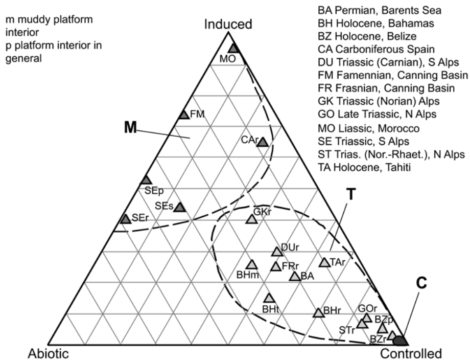
Fig. 3: Proportions of abiotic, biotically induced and biotically controlled material in factory output estimated from the composition of some well-known Phanerozoic limestone formations. C factory consists almost entirely of one category, i. e. biotically controlled precipitates. M and T factories are mixtures of all three categories with M factory richer in bio-induced and abiotic material, T factory richer in biotically controlled material. After Schlager (2005), modified.
