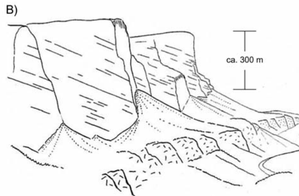
Fig. 7: Effect of sediment grain size on morphology of submarine slopes. A) Slope of extant platform dominated by muddy, cohesive sediment. Note low slope angle and indications of slumping. Line drawing from seismic profile, northern flank of Little Bahama Bank. B). Prograding carbonate platform slope composed of sand, rubble and over 50% of automicrite lenses and layers. Despite its abundance, automicrite was not able to build morphologically significant mounds; slope morphology is controlled by the angle of repose of the detrital material. Note similarity of Triassic slope angles with angle of modern scree, also composed of rubble and sand (difference between subaerial and subaquatic angles of repose of coarse material is very small). After Kenter (1990) and Schlager (2005), modified.
