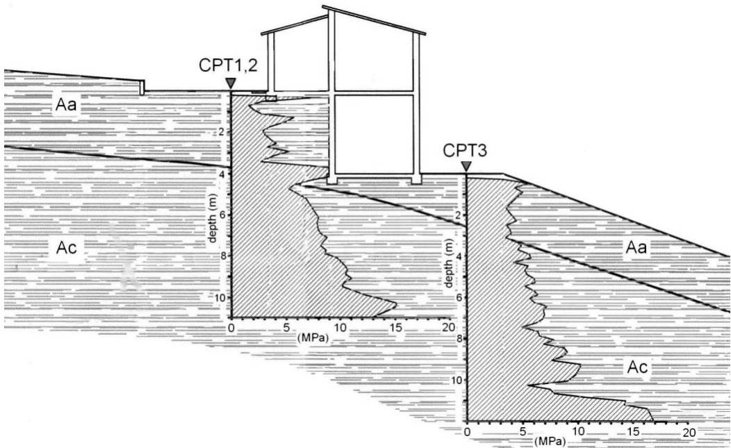
Fig. 6: Soil profile and CPT initial results.
