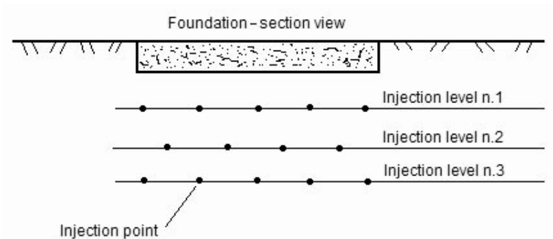
Fig. 3: Schematic representation of the Uretex injection procedure.
